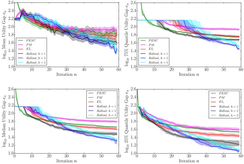
Figure 6: Mean (top left), 75% quantile (top right), median (bottom left) and 25% quantiles of the utility gap for P3.
