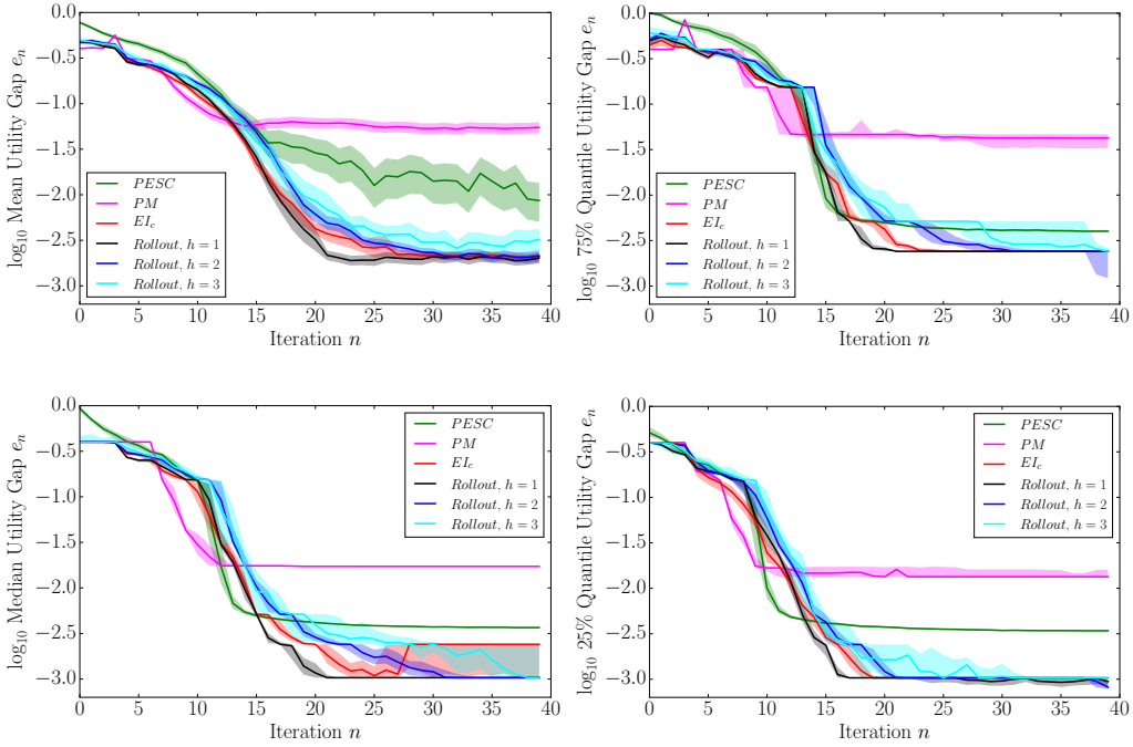
Figure 5: Mean (top left), 75% quantile (top right), median (bottom left) and 25% quantiles of the utility gap for P2.
