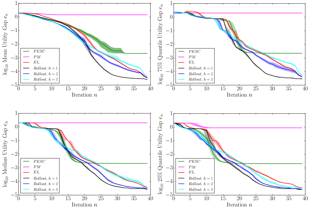
Figure 4: Mean (top left), 75% quantile (top right), median (bottom left) and 25% quantiles of the utility gap for P1.
