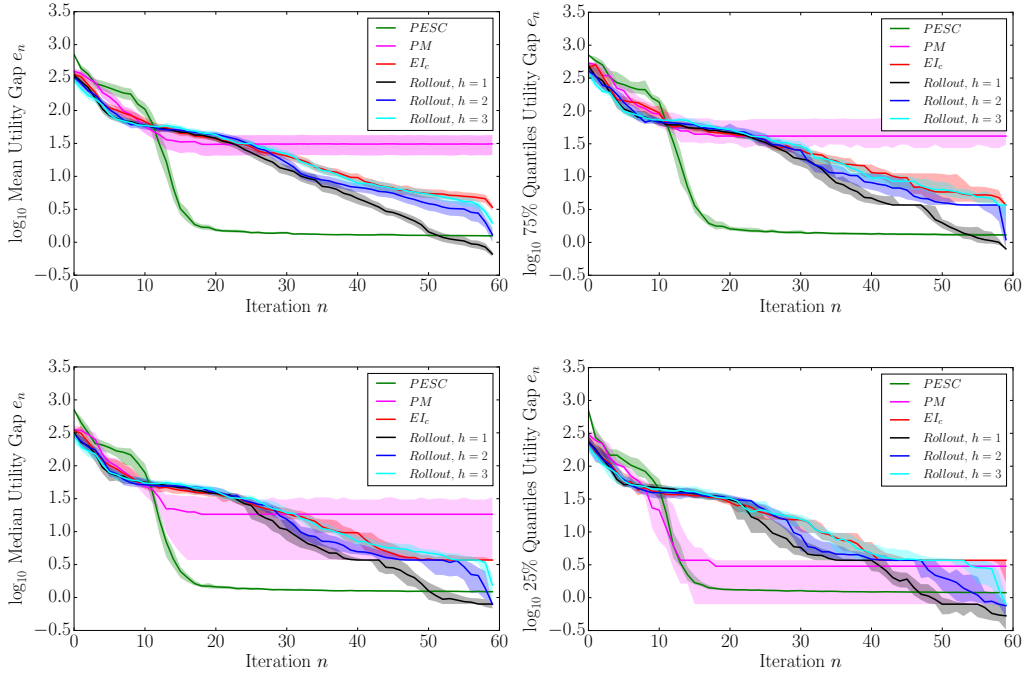
Figure 7: Mean (top left), 75% quantile (top right), median (bottom left) and 25% quantiles of the utility gap for P4.
