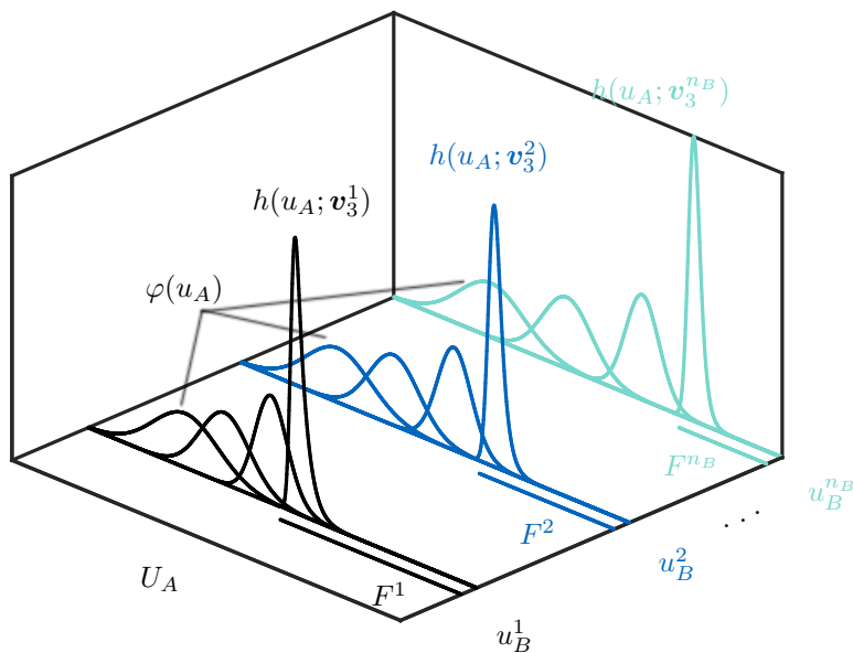
Figure 1: Illustration of iCE densities: h(u_A; \mathbf{v}_i^j) is the importance density used at the i -th iCE step in the j -th conditional reliability problem in standard-normal space. Intermediate densities at equal iCE-steps i associated with different conditional reliability problems j tend to look identical in this illustration but are generally not. An exception is the nominal density \varphi(u_A) , which is identical for each problem.
