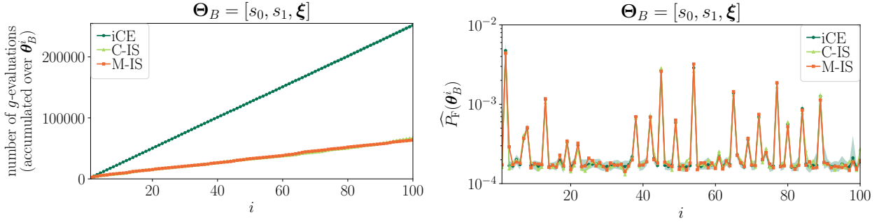
Figure 12: Monopile configuration 1: computational cost (left) and conditional failure probability estimates at \Theta_B samples (right) with iCE reference solution mean and 95% CI.
