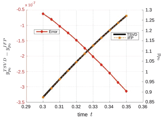
Fig. 6.8 The (left ordinate axis) error between the prediction outputs from the TSVD and IFP approaches (red, diamonds) and the (right ordinate axis) predictions themselves based on TSVD (black, solid) and IFP (orange, dashed, squares) approaches.
