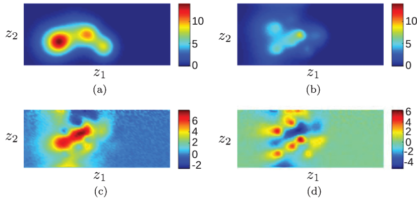
Fig. 6.12 The (a) real initial condition, (b) Tikhonov-regularized estimate, (c) IFP estimate, and (d) error \mu_e = \mu^{TR} - \mu^{IFP} . In Figure 6.13 we show the propagation of \mu_e to the output time steps.
