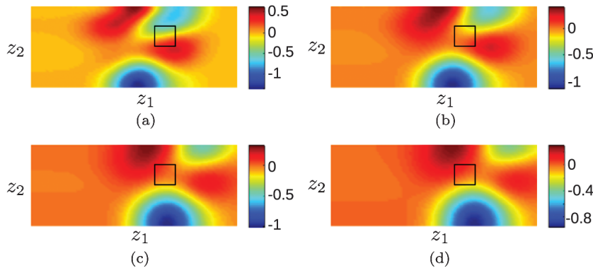
Fig. 6.13 The propagation of \mu_e according to the advection-diffusion equation to the prediction output y_{p_1} at time steps (a) t = 25\Delta t , (b) t = 35\Delta t , (c) t = 45\Delta t , and (d) t = 50\Delta t . The average concentration inside of \Omega_1 (box) is negligible for all time steps t \in [25\Delta t, 50\Delta t] .
