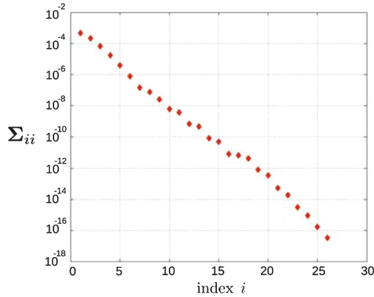
Fig. 6.11 The singular values on the diagonal of \Sigma reflecting the joint measure of experiment and prediction observability for the Tikhonov-regularized inverse problem approach.
