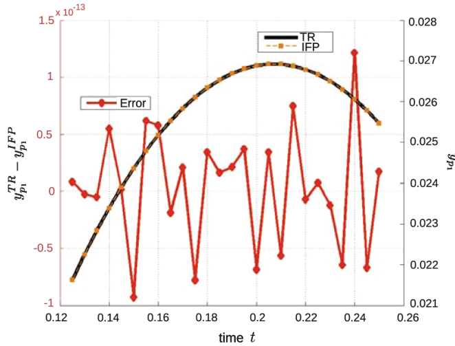
Fig. 6.14 The (left ordinate axis) error between the prediction outputs from the Tikhonov-regularized and IFP approaches (red, diamonds) and the (right ordinate axis) predictions themselves based on Tikhonov-regularized (black, solid) and IFP (orange, dashed, squares) approaches.
