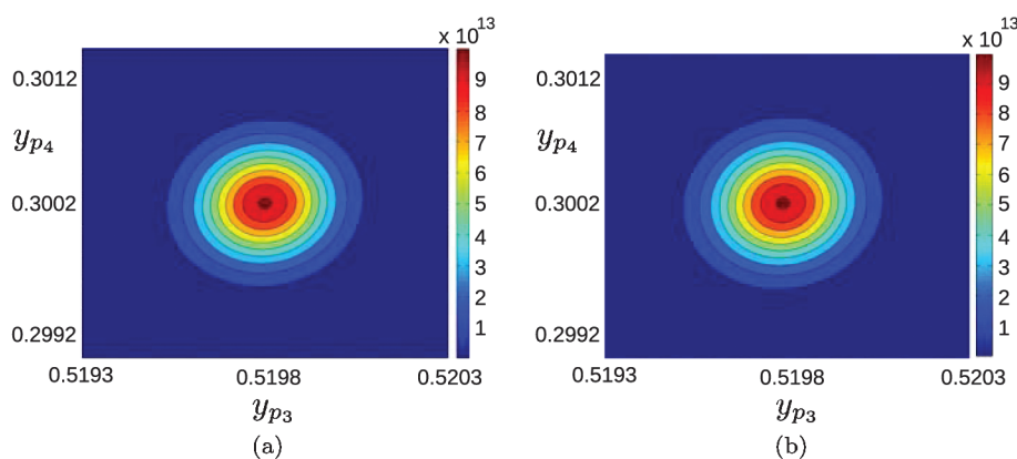
Fig. 6.16 Contour plots of the joint probability density function over the outputs (y_{p_3}, y_{p_4}) for the (a) traditional approach and the (b) IFP approach. The means and covariance matrices corresponding to both approaches are also given in Table 6.2.
